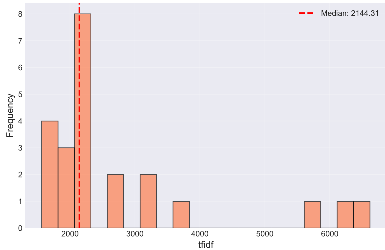
tfidf Distribution
