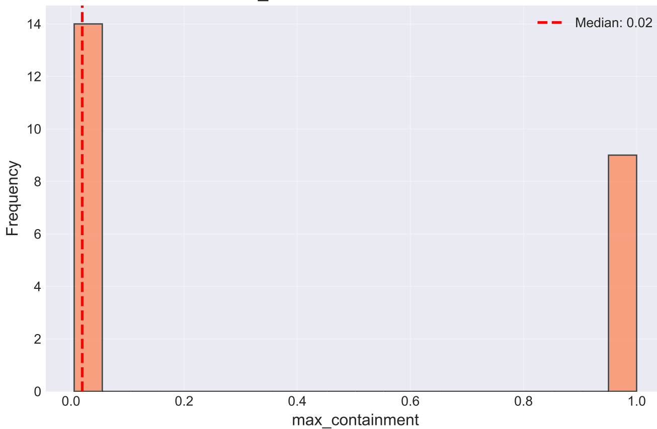
max_containment Distribution
