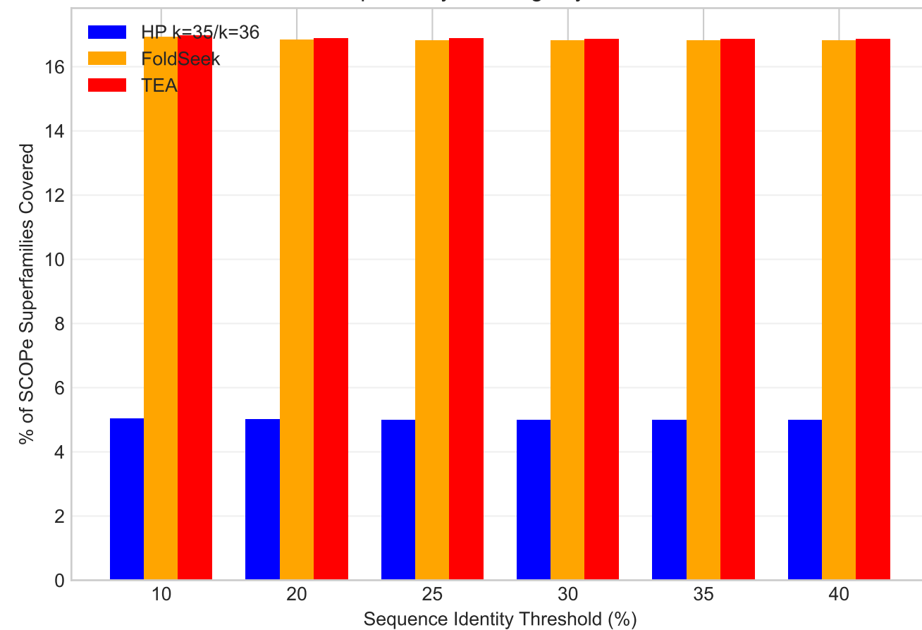
HP Relative Performance vs FoldSeek/TEA
