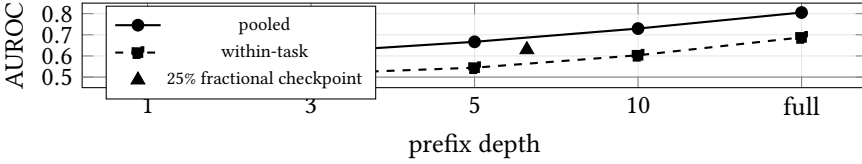
Fig. 1. The reimplemented published monitor on C1 (79,929 trajectories, 926 mixed units). The x-axis is categorical with equal spacing; “full” is the completed trajectory. Pooled AUROC overstates within-task discrimination by +0.06–0.13 at every depth; run-level signal is within resolution of chance at one turn and real only late. The fractional checkpoint (triangle, placed at its mean observed depth of 6.6 turns) sits above the within-task curve—the leakage of Figure 2.
