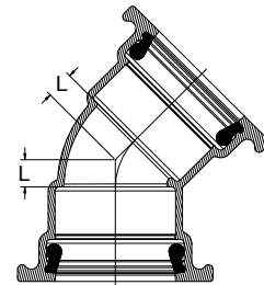
45° BEND DIOD x DIOD (G x G)
