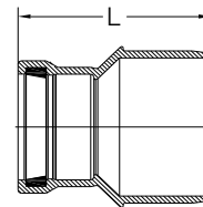
CONCENTRIC INCREASER (G x S)
