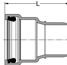
ADAPTER DIOD x SEWER (G x S)
