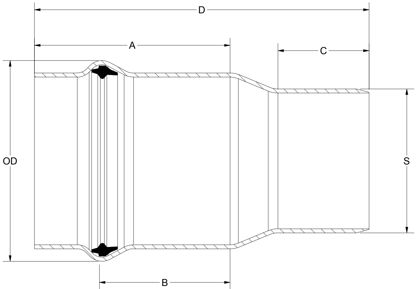
4" - 8" ADAPTER, C900xSEWER, GxS, SDR35
