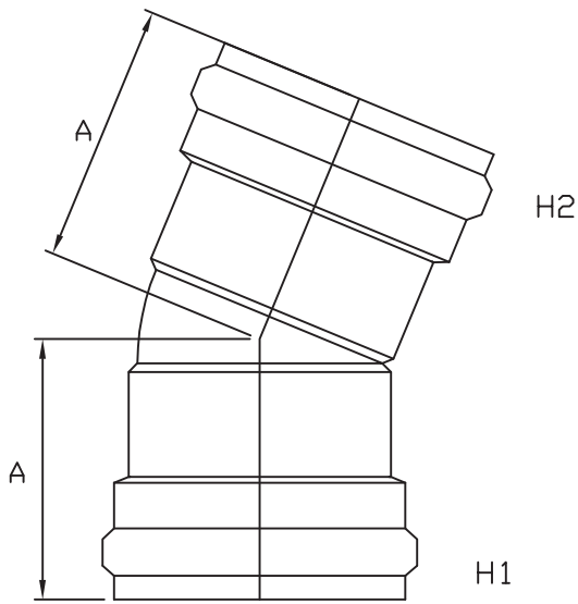
INJECTION MOLDED FITTING (M+)
