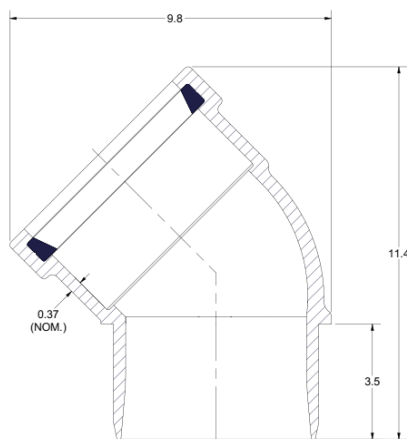
6" 45 Bend GxS
