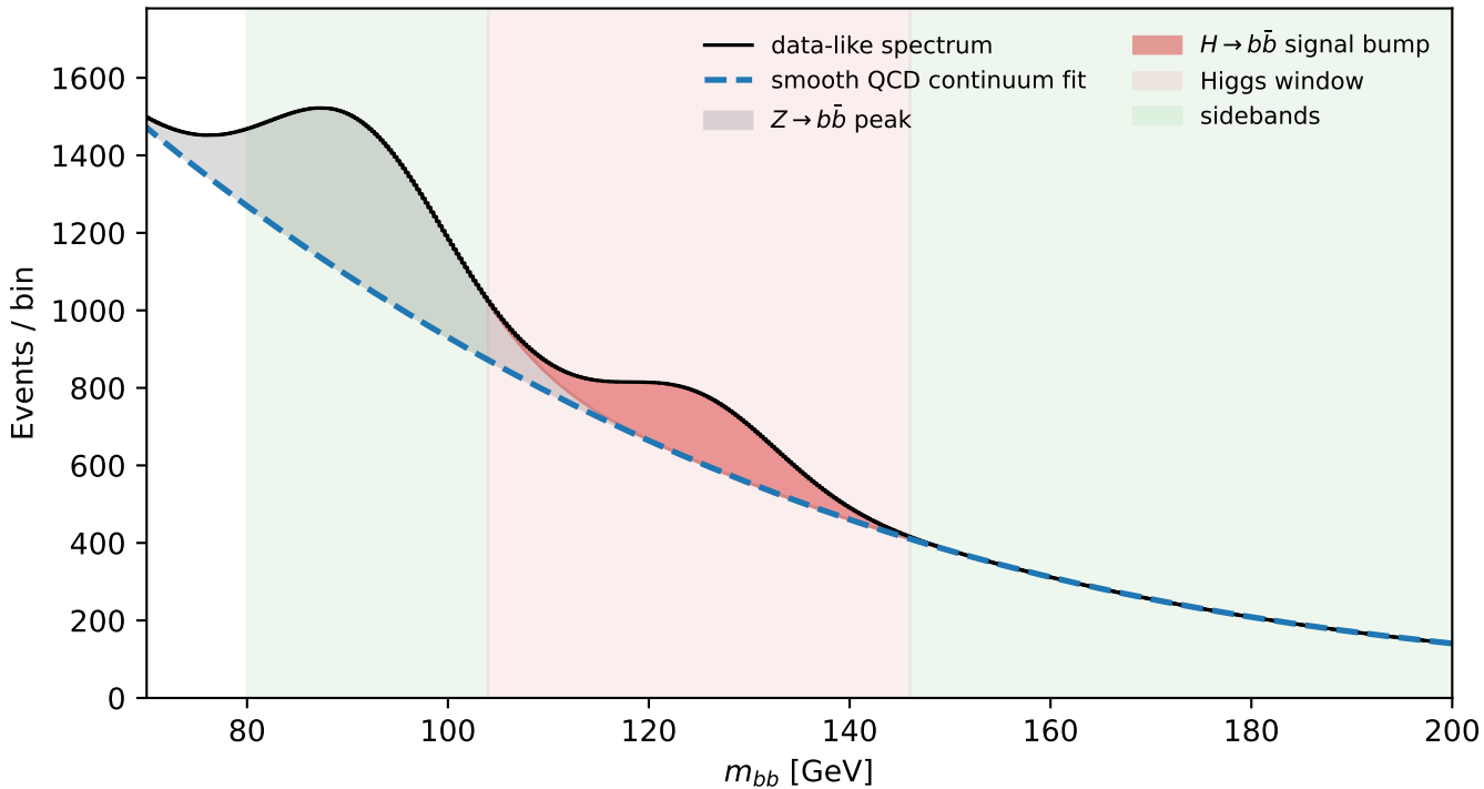
Smooth continuum fit: CMS-style VBF H \rightarrow b\bar{b} multijet model
