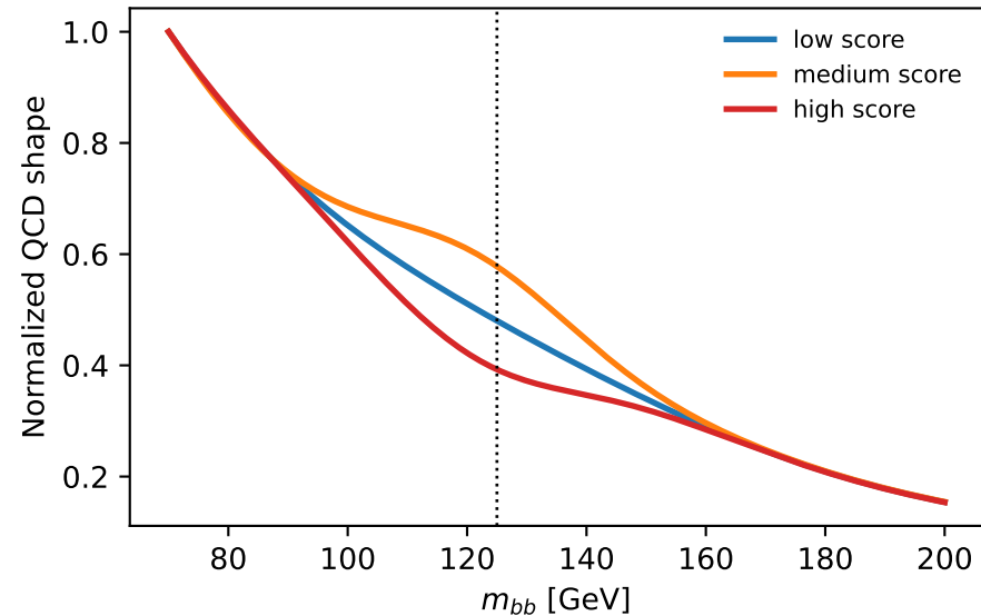
Ordinary classifier can sculpt mass
