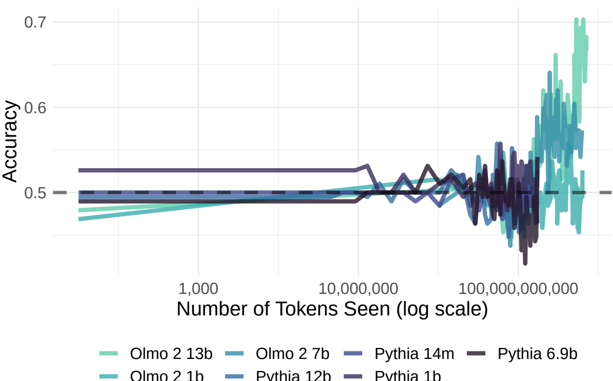
False Belief Task Accuracy Over Pretraining
