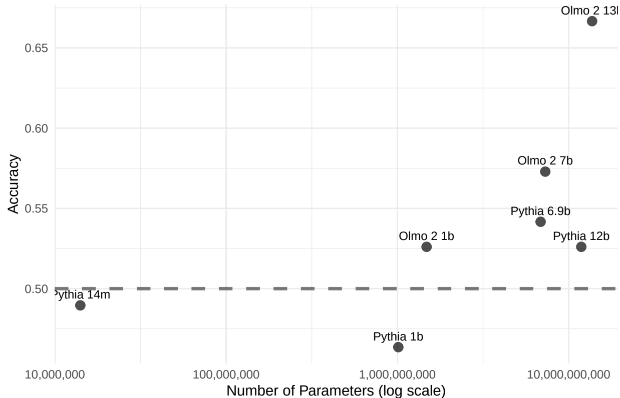
False Belief Task Accuracy at Final Step
