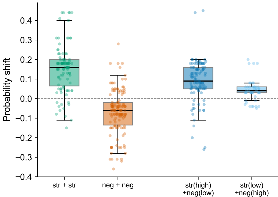
Compound probe shift by direction pairing
