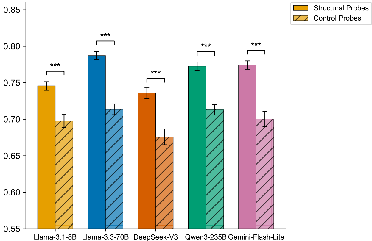
Within-Question Cosine Similarity
