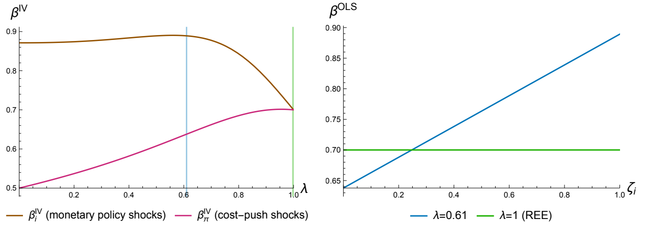
(a) Conditional sensitivities \beta_i^{IV} and \beta_\pi^{IV} as functions of (b) Unconditional sensitivity \beta^{OLS} as a function of relative importance of monetary policy shocks \zeta_i
