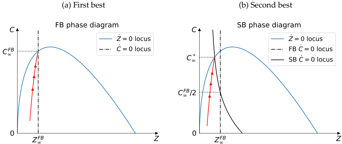
Figure 4: Phase diagram
