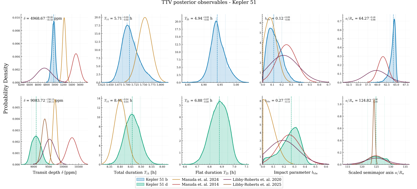
Figure 2. Marginal posterior distributions of the observables for Kepler-51b (top row) and Kepler-51d (bottom row) obtained from the TTV analysis carried out in this work are shown as filled distributions. Vertical dashed lines and the accompanying labels indicate the median and the 68% credible interval for each marginal posterior. For comparison, literature estimates are depicted as normal distributions (unfilled curves) constructed from the published point values and their reported uncertainties; in the case of K. Masuda et al. (2024) , a truncated normal distribution is used for the impact parameter b to respect its physical limits. Only those observables provided by each reference are plotted (for example, none of the alternative sources report values for the flat-bottom duration T_{23} ).
