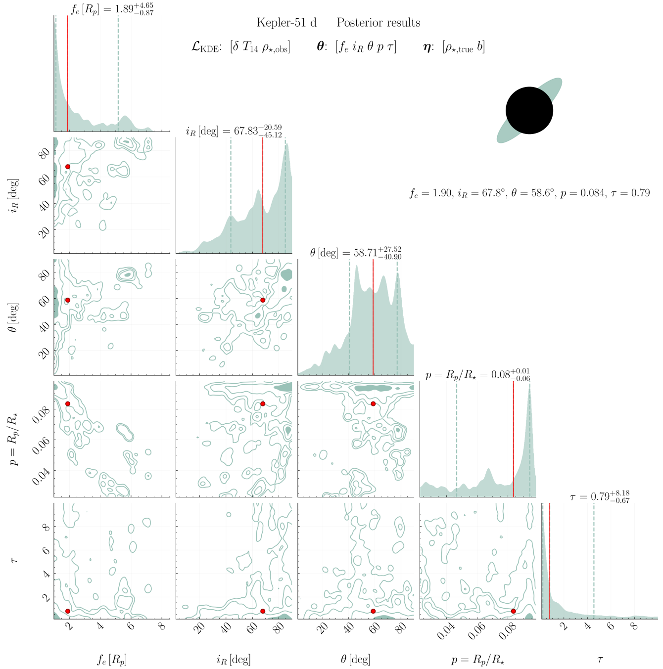
Figure 5. Posterior joint distribution for the PR inference of Kepler-51d for a chosen retrieval scenario (see text). The figure specifications are identical to those in Figure 4.
