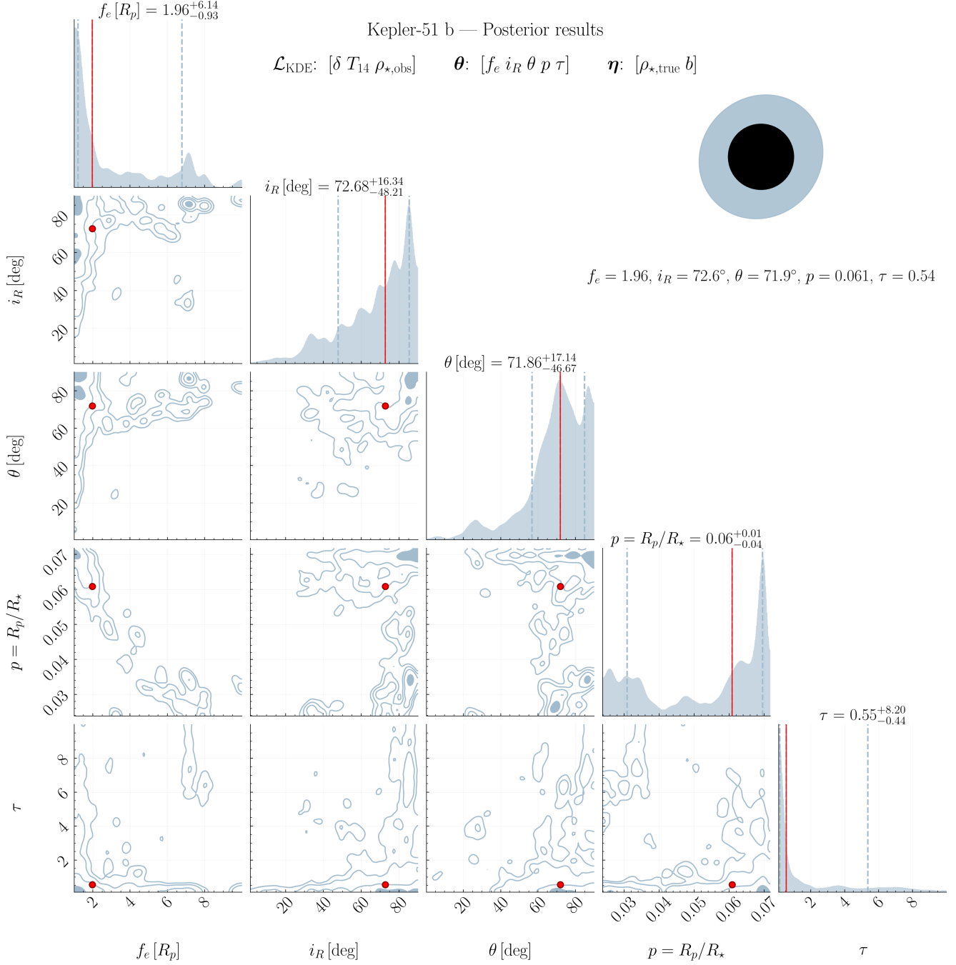
Figure 4. Posterior joint distribution for the PR inference of Kepler-51b for a chosen retrieval scenario (see text). The corner-plot panels display 2D and 1D marginal posteriors for both the ringed planet parameters and the nuisance parameters. For visualization, we include a schematic of the ring system constructed from the median values of the marginal posteriors, indicated by red lines on the 1D marginals. The dark disk denotes the planet, while the filled elliptical annulus represents the ring. Red dots on the panels indicate where the ringed planet parameter is positioned that matches the schematic illustration.
