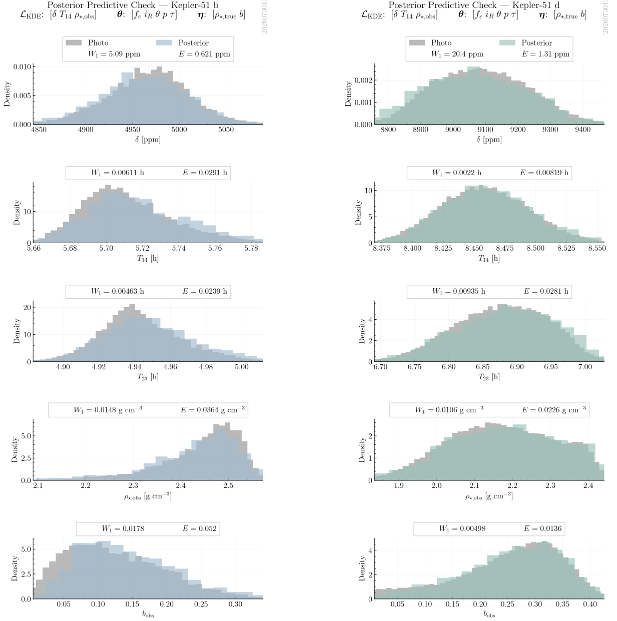
Figure 6. Posterior predictive checks (PPCs) for Kepler-51b and Kepler-51d in the fully free retrieval scenario. PPCs compare the model-predicted distribution (blue) with the photometrically derived posterior (grey) for each transit observable. The reported values of W_1 and E quantify the self-consistent goodness-of-fit between the ringed-planet model and the observed transit observables.
