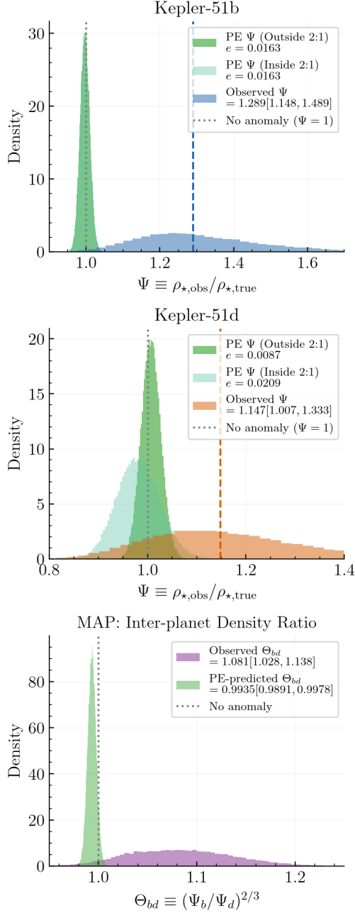
Figure 5. Forward prediction of the photoeccentric bias \Psi(e, \omega) versus the observed density anomaly \Psi . Using dynamical posteriors from K. Masuda et al. (2024), the induced biases for Kepler-51b (top panel) and Kepler-51d (middle panel) are \lesssim 1\% , failing to reproduce the large observed anomalies. The Multibody Asterodensity Profiling (MAP) analysis (bottom panel) independently demonstrates that the photoeccentric prediction for the inter-planet density ratio \Psi(b)/\Psi(d) is severely incompatible with the observed differential anomaly.
