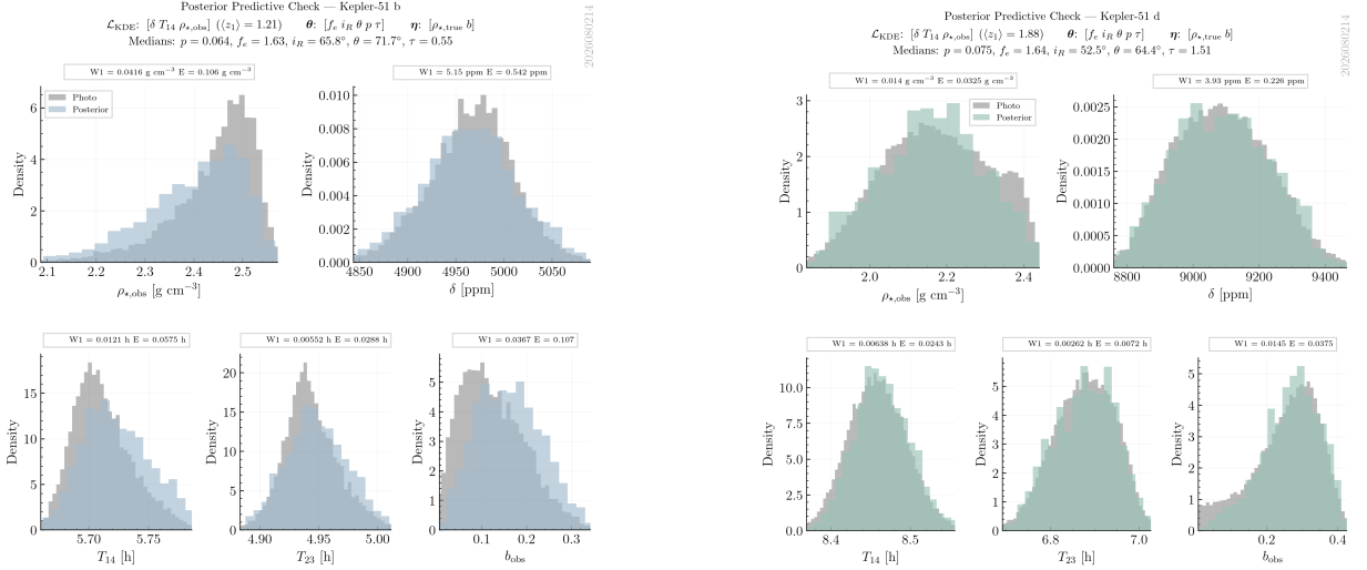
Figure 8. Posterior predictive checks (PPCs) for Kepler-51b and Kepler-51d in the fully free retrieval setup. PPCs compare the model-predicted distribution (blue) with the photometrically derived posterior (grey) for each transit observable. The reported values of W_1 and E quantify the self-consistent goodness-of-fit between the ringed-planet model and the observed transit observables.
