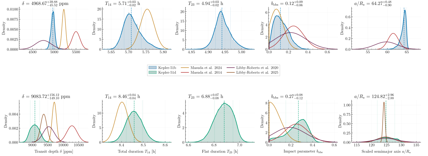
Figure 2. Marginal posterior distributions of the observables for Kepler-51b (top row) and Kepler-51d (bottom row). Those obtained from the PhotoFIT carried out in this work are shown as filled distributions. Vertical dashed lines and the accompanying labels indicate the median and the 68% credible interval for each marginal posterior. For comparison, literature estimates are depicted as normal distributions (unfilled curves) constructed from the published point values and their reported uncertainties; in the case of K. Masuda et al. (2024), a truncated normal distribution is used for the impact parameter b to respect its physical limits. Only those observables provided by each reference are plotted (for example, none of the literature sources report values for the flat-bottom duration T_{23} ).
