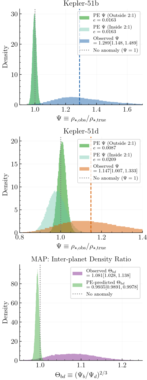
Figure 5. Top panels: Forward prediction of the photoeccentric bias \Psi^{\text{PE}}(e, \omega) versus the observed density anomaly \Psi , using dynamical posteriors from K. Masuda et al. (2024). Bottom panel: The Multibody Asterodensity Profiling (MAP) analysis which compares the expected inter-planet density ratio \Theta_{bd} = (\Psi_b / \Psi_d)^{2/3} to the observed one.
