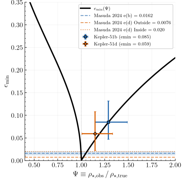
Figure 4. The minimum required eccentricity e_{\min} plotted as a function of the density ratio \Psi = \rho_{\star, \text{obs}} / \rho_{\star, \text{true}} (solid black curve). The dashed curves show the actual eccentricity values obtained from the detailed TTV analysis by K. Masuda et al. (2024).
