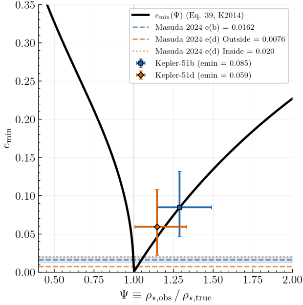
Figure 4. The minimum required eccentricity e_{\min} plotted as a function of the density ratio \Psi = \rho_{\star,\text{obs}}/\rho_{\star,\text{true}} (solid black curve). The dashed curves show the actual eccentricity values obtained from the detailed TTV analysis by K. Masuda et al. (2024).
