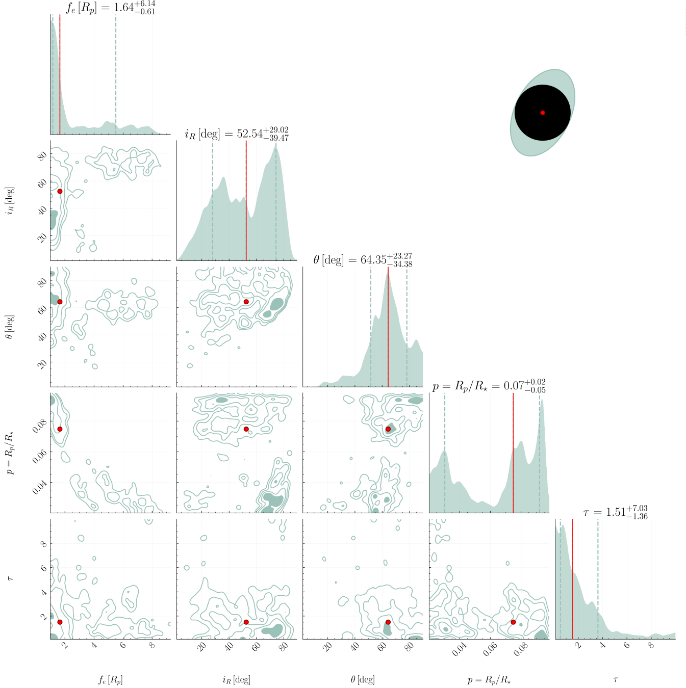
Figure 5. Posterior joint distribution for the PR inference of Kepler-51d for a chosen retrieval setup (see text). The figure specifications are identical to those in Figure 4.
