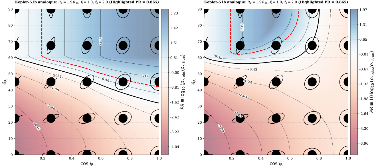
Figure 7. Comparison of the PhotoRing effect contours for Kepler-51b using the original exorings analytical approximation from J. I. Zuluaga et al. (2015) (left) and the precise semi-analytical model geotrans (right). The original model exhibits geometrical artifacts at certain high projected tilts and inclinations. You can compare the panel on the right with Figure 1, which was obtained using the refined analytical model presented in this appendix.
