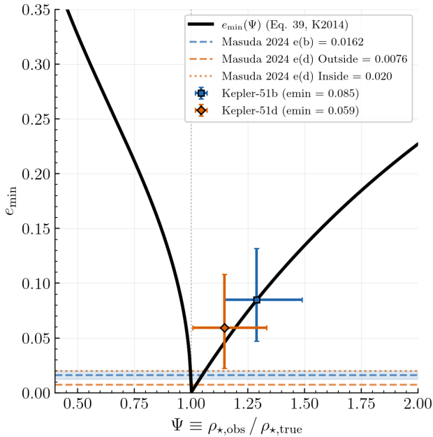
Figure 4. The minimum required eccentricity e_{\min} plotted as a function of the density ratio \Psi = \rho_{*,\text{obs}}/\rho_{*,\text{true}} (solid black curve). The dashed curves show the actual eccentricity values obtained from the detailed TTV analysis by K. Masuda et al. (2024).
