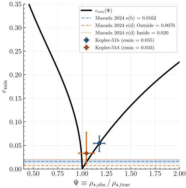
Figure 3. The minimum required eccentricity e_{\min} plotted as a function of the density ratio \Psi = \rho_{*,\text{obs}}/\rho_{*,\text{true}} (solid black curve). The dashed curves show the actual eccentricity values obtained from the detailed TTV analysis by K. Masuda et al. (2024).
