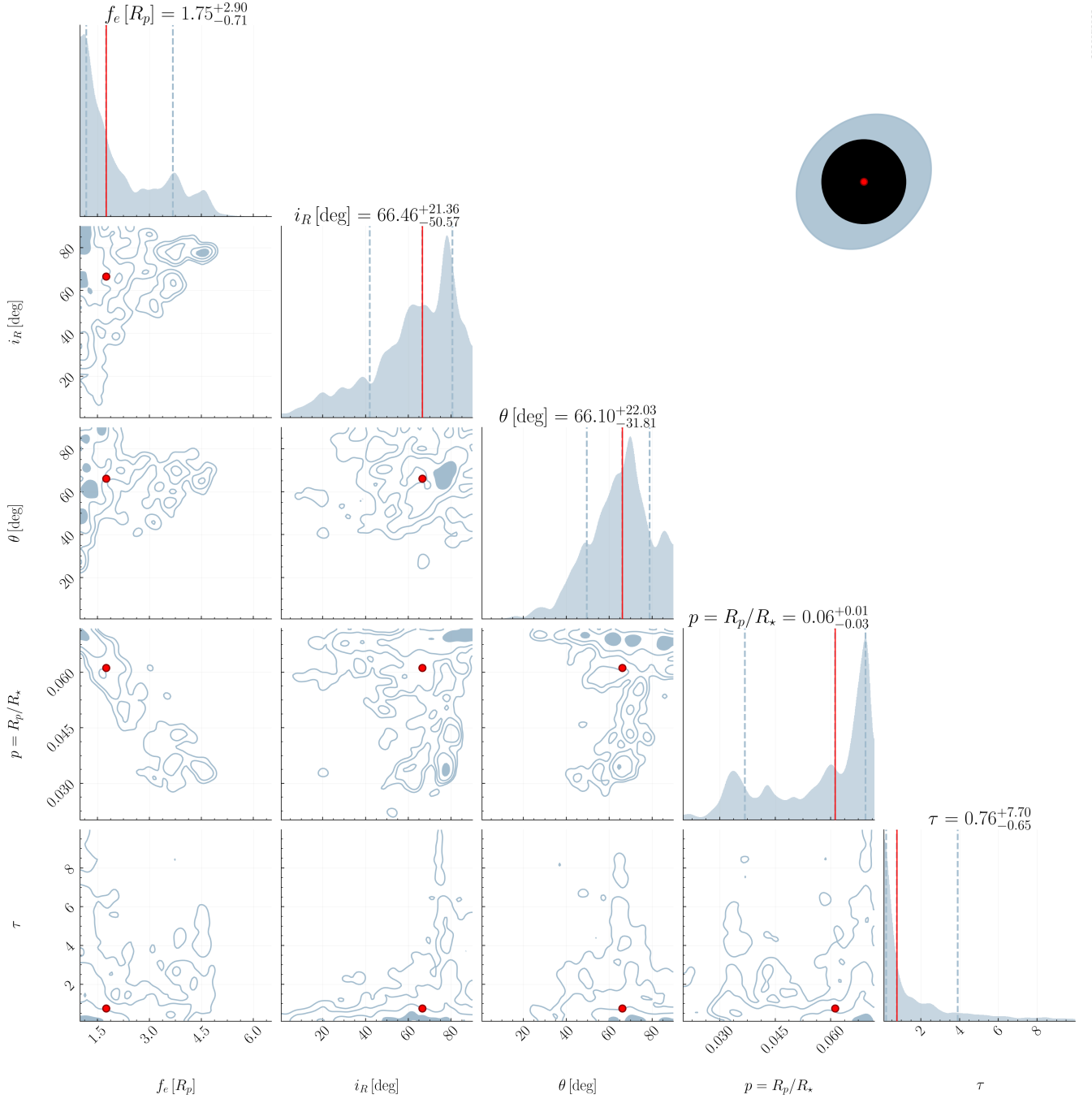
Figure 4. Posterior joint distribution for the PR inference of Kepler-51b for a chosen retrieval setup (see text). The corner-plot panels display 2D and 1D marginal posteriors for both the ringed planet parameters and the nuisance parameters. For visualization, we include a schematic of the ring system constructed from the median values of the marginal posteriors, indicated by red lines on the 1D marginals. The dark disk denotes the planet, while the filled elliptical annulus represents the ring. Red dots on the panels indicate where the ringed planet parameter is positioned that matches the schematic illustration.
