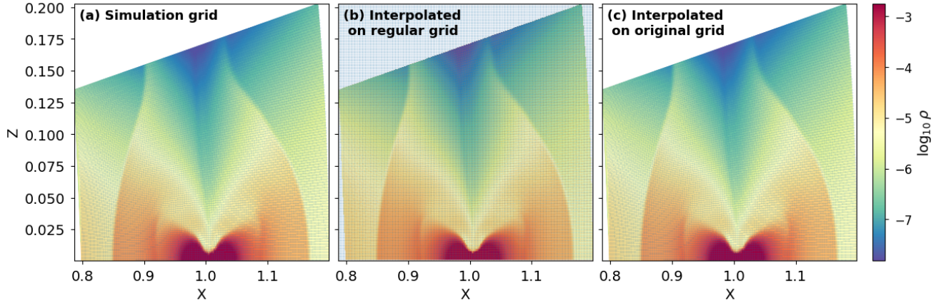
Figure 1: Visual comparison of the density field in the meridional slice under consideration. Left: original density field defined on the irregular simulation mesh. Center: field interpolated onto a high-resolution regular Cartesian grid. Right: field reconstructed on the original mesh after the round-trip process. All three panels are shown with the same normalization in \log_{10} \rho . The interpolation preserves the global morphology of the field, including the vertical stratification of the disk and the structures associated with the planetary gravitational well, without introducing spatial artifacts.
