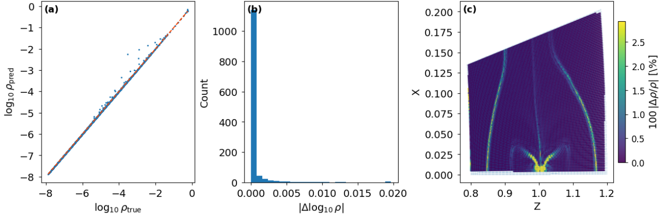
Figure 2: Quantitative diagnostics of the round-trip test applied to the density field. Left: scatter plot between the reconstructed field \rho_{\text{back}} and the original field \rho_{\text{true}} in logarithmic scale; the dashed line indicates the identity relation. Center: distribution of |\Delta \log_{10} \rho| , which shows a strong concentration at small values. Right: spatial map of the absolute relative error 100 |\rho_{\text{back}} - \rho_{\text{true}}| / \rho_{\text{true}} , expressed as a percentage. The largest discrepancies are concentrated in regions with sharp spatial gradients, such as the vicinity of the mid-plane and the structures associated with shocks. Although these discrepancies are relatively larger compared to the rest of the domain, their absolute magnitude is small and they do not give rise to extended regions.
