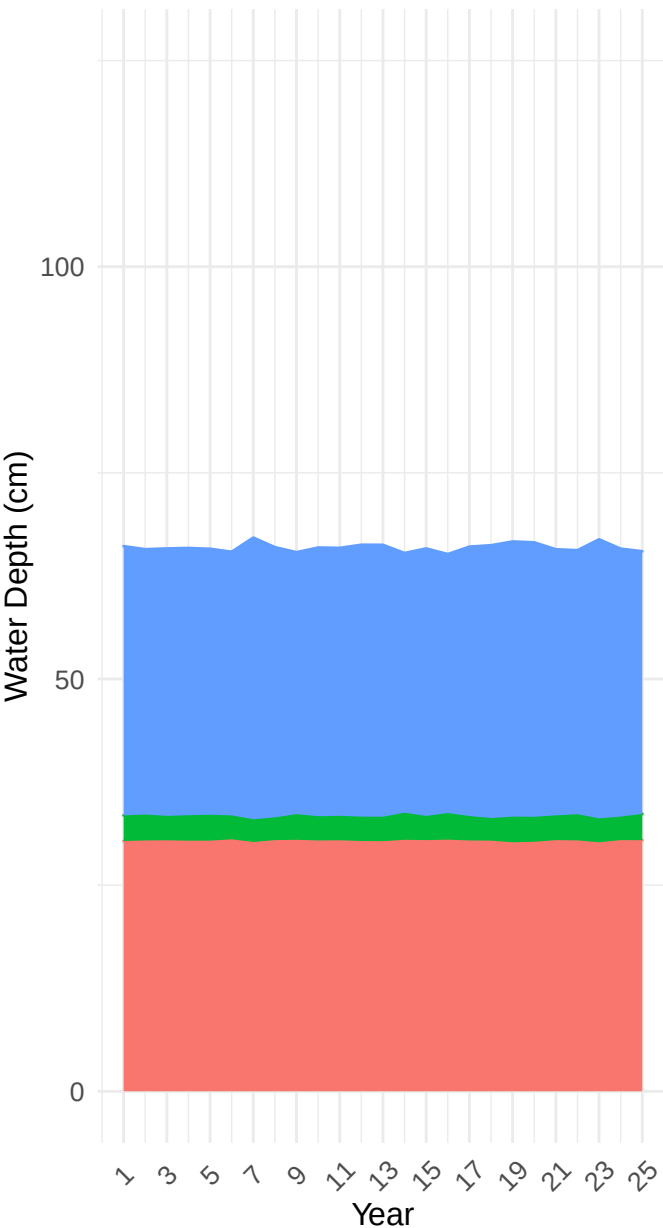
Dry Climate Deterministic
