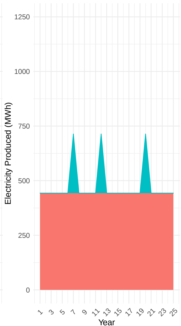
SI-EP Dry-Moderate Climate Res
