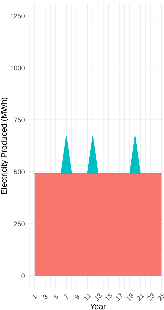
SI-EP Dry-Moderate Climate Deterministic
