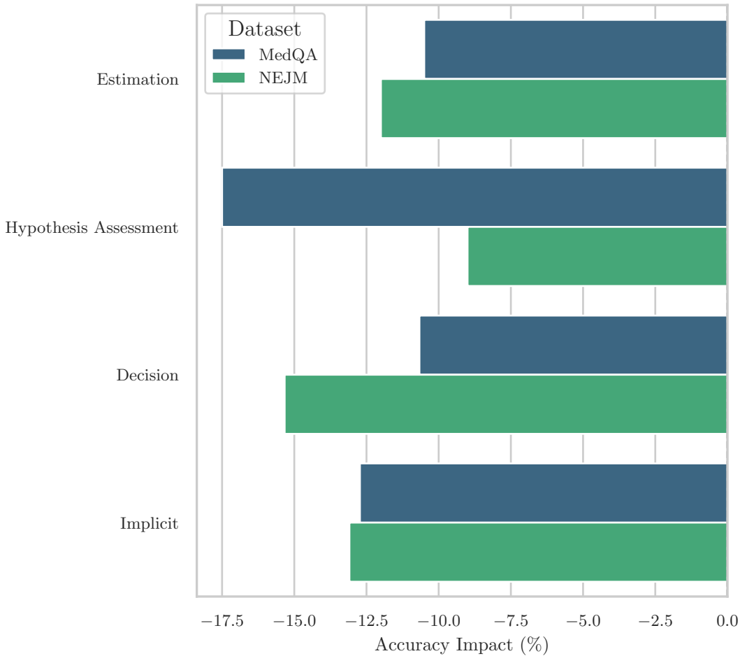
Bias Category
