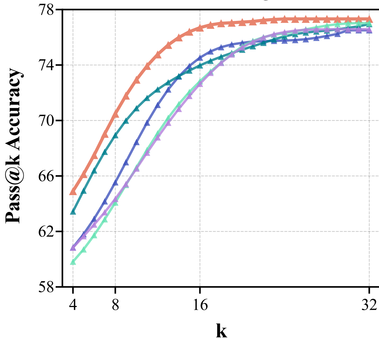
RealWorldQA
