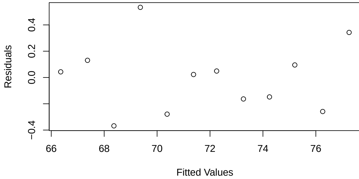
Residual Plot: Height vs Predicted Height
