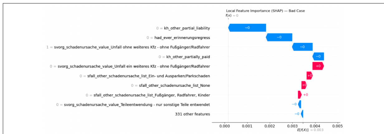
Abb. 11: Feature Importance (SHAP) im Bad Case.
