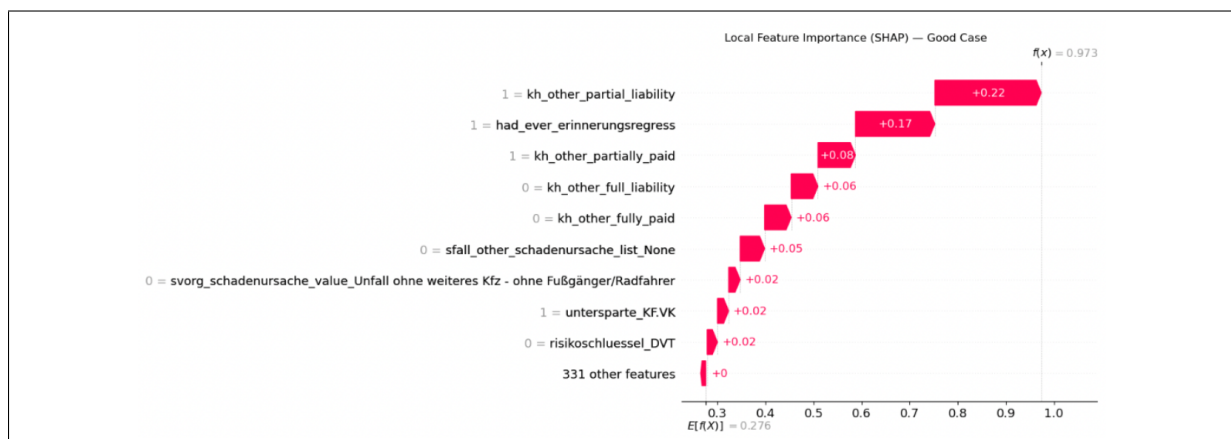
Abb. 9: Feature Importance (SHAP) im Good Case.
