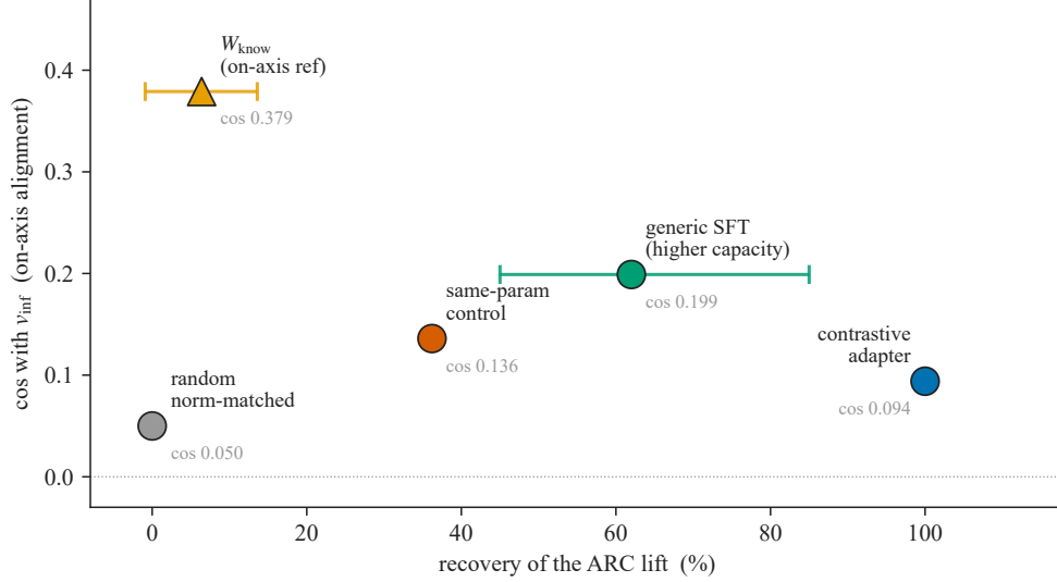
Figure 1: The matched-control spectrum on two independent axes. x : fraction of the ARC lift each direction recovers; y : cosine with the functional correctness direction v_{inf} (net effect on activations for the four methods; the reference direction itself for W_{know} , marked \blacktriangle ). The two orderings are not monotone in each other: the most on-axis point ( W_{know} , \cos 0.379 ) recovers only 6.4%, while the top recoverer (the contrastive adapter, 100%) is the least on-axis ( \cos 0.094 ). The two non-contrastive controls separate the two factors at work. The same-parameterization control (identical 48 head-pairs and 12,336 parameters; only the objective differs) recovers \sim 37\% at \cos 0.136 , while higher-capacity generic SFT (1,800 \times –117,000 \times more parameters) recovers \sim 62\% at \cos 0.199 : with the parameterization held fixed the contrastive objective is both further off-axis and far more effective, whereas added capacity buys recovery while moving toward the axis. So how much a generic objective recovers depends on capacity, and where the recovery lives depends on the objective — two factors, not one ordered scale. Horizontal bars are the published 95% intervals on the recovery fraction where one exists — W_{know} [-0.9\%, +13.6\%] and generic SFT [45\%, 85\%] ; the random floor (three seeds), the same-parameterization control (three seeds, sd 5.0 pp) and the contrastive anchor (100% by construction) carry none, and we do not synthesise one. W_{know} ’s interval crosses zero and overlaps the random floor: its 6.4% is statistically indistinguishable from no recovery (exact McNemar p = 0.136 ), and it is counted with the floor rather than as a rung. Values in Table 8.
