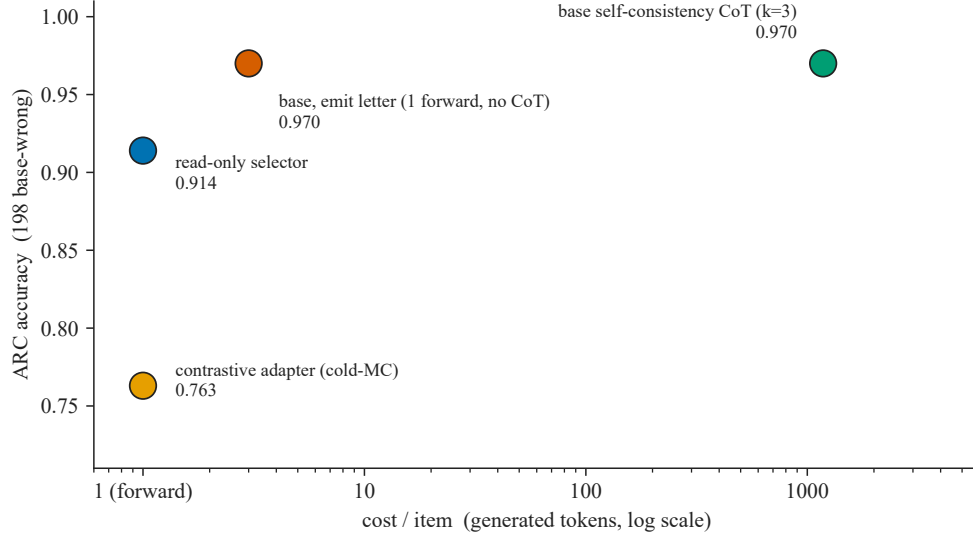
Figure 2: The deployment triangle on the 198 base-wrong ARC items. x : cost per item in generated tokens (log scale; a single forward is one unit); y : ARC accuracy. Four routes: the contrastive adapter’s cold-MC scoring (0.763, one forward) is dominated by everything; the read-only selector (0.914, one forward) improves on it read-only; the base asked to emit the answer letter in one forward (0.970) matches the reasoning baseline at \sim 1000\times less cost and dominates both the adapter and the selector at equal cost ; base self-consistency CoT (0.970, \sim 1179 tokens) ties letter-emission at far higher cost. The whole LoFiT/ITI-for-cold-MC family optimizes a readout that the most trivial same-cost alternative — ask the base for the letter — already beats. The comparison is evidentiary, not a like-for-like scoring test: letter emission is a different (lettered-MCQ) readout than the cold-MC channel (Section 3.2), so the triangle contrasts two readouts of the same base at equal cost — the lossy-readout thesis in its sharpest form — and the selector’s role stays evidentiary (read \neq write), not a deployment recommendation, since even it is dominated by letter emission.
