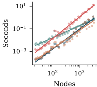
Runtime by stage
