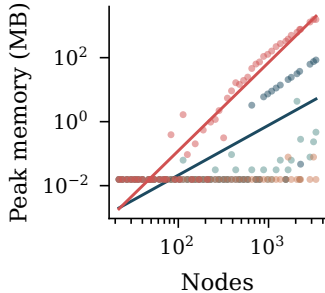
Memory by stage
