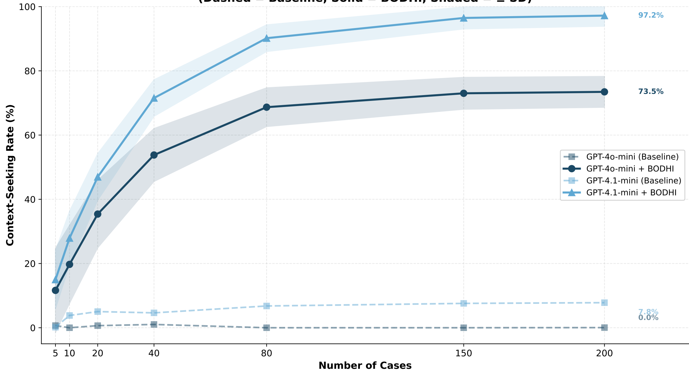
Context-Seeking Rate Convergence: Baseline vs BODHI (Dashed = Baseline, Solid = BODHI, Shaded = \pm SD)
