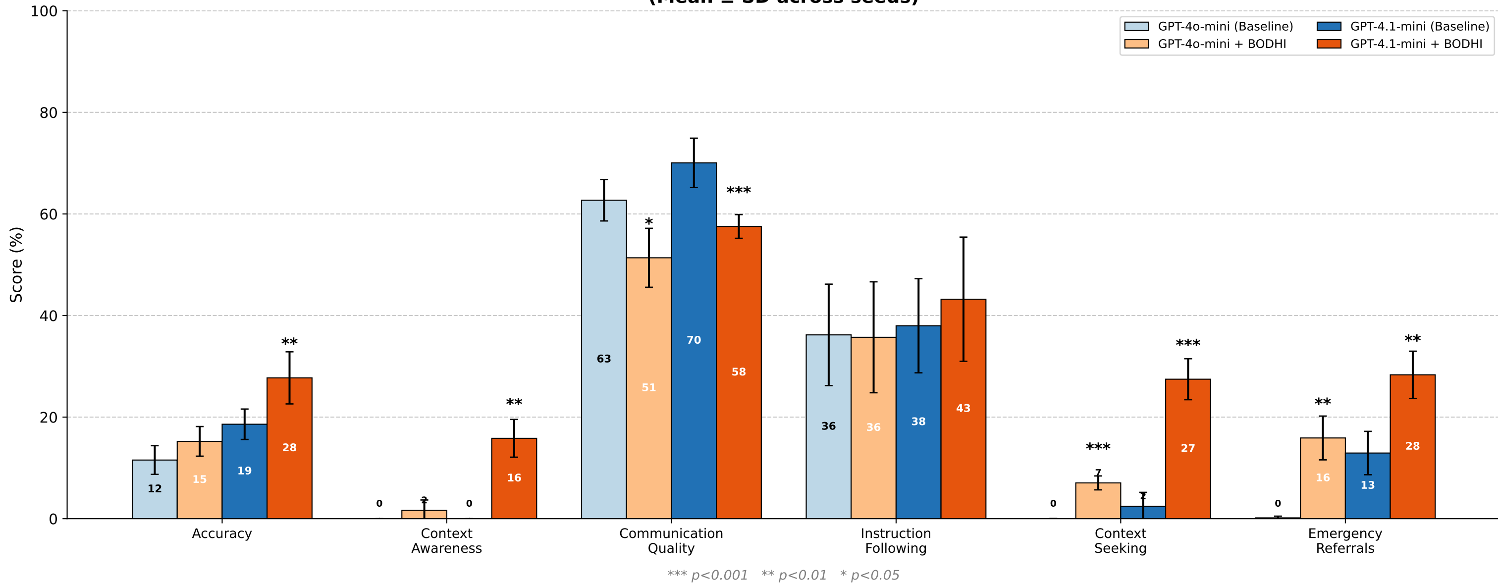
Multi-Metric Comparison: Baseline vs BODHI by Model (Mean \pm SD across seeds)
