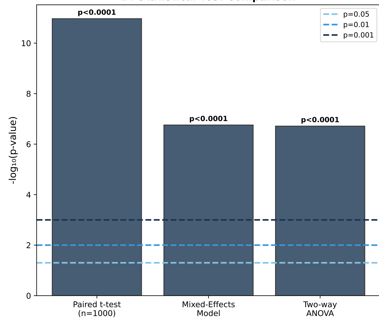
D. Statistical Test Comparison
