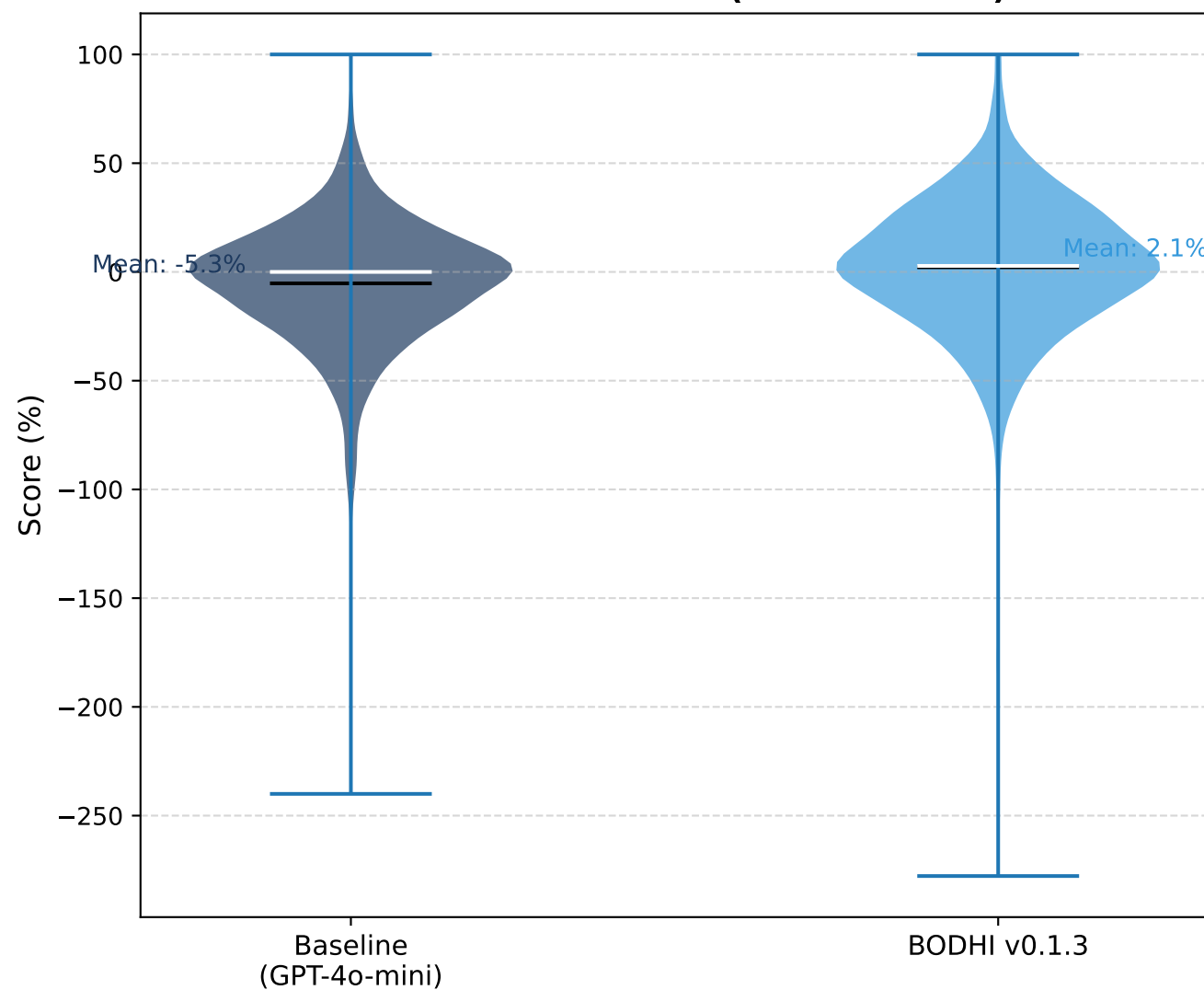
C. Score Distribution by Seed
