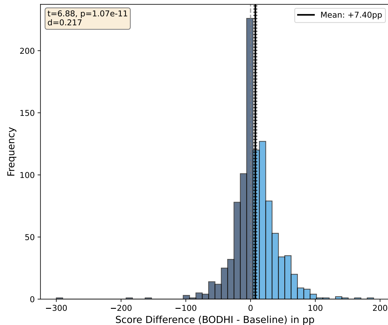
D. Statistical Test Comparison
