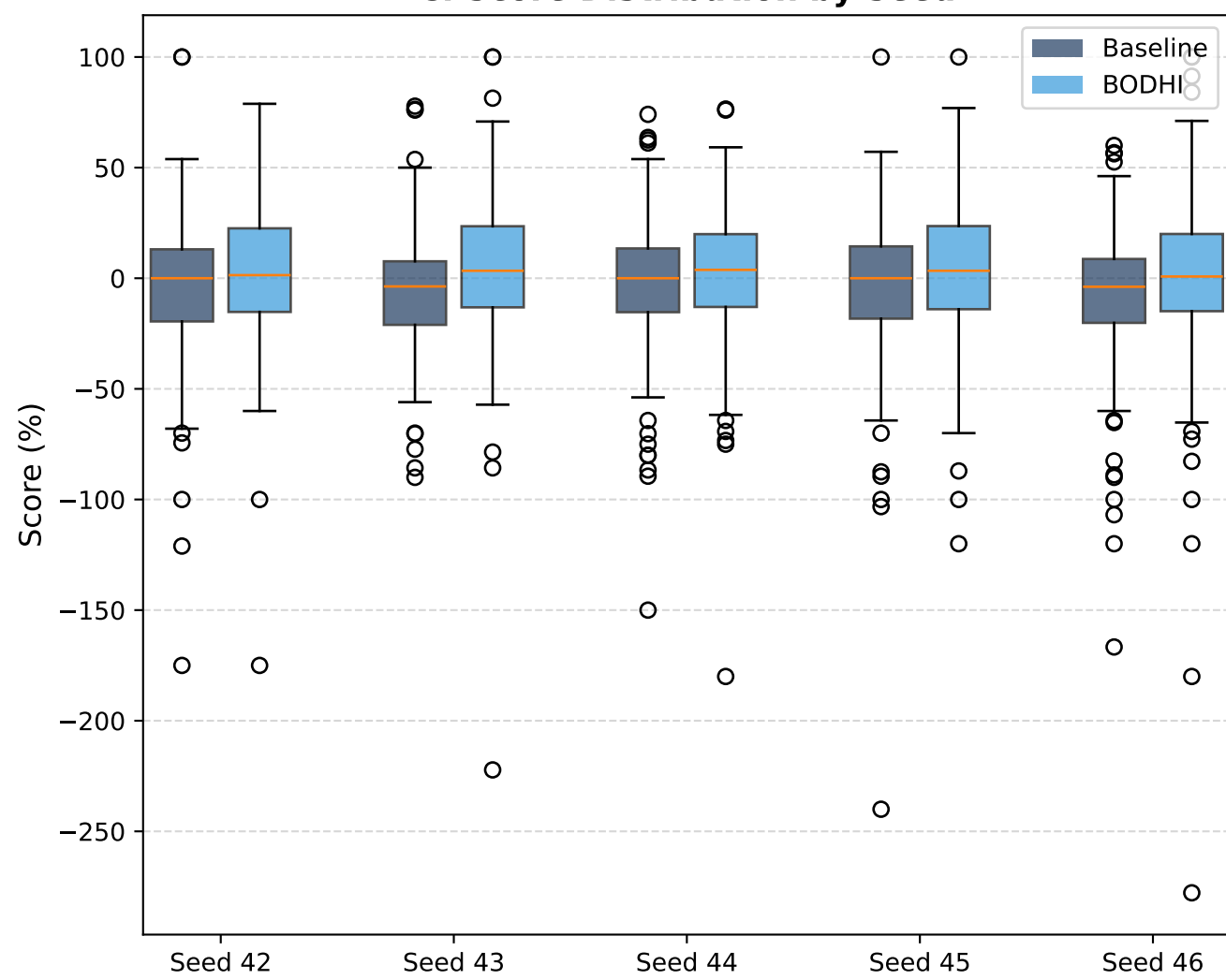
C. Score Distribution by Seed
