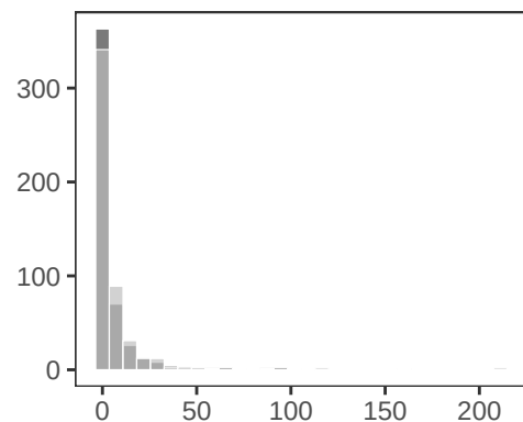
Log-normal
