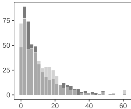
Chi-squared
