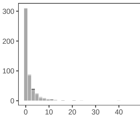
Weibull
