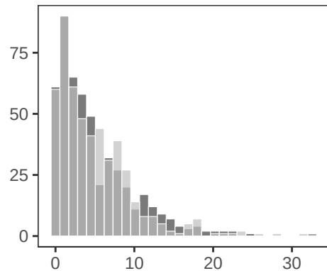
Log-normal
