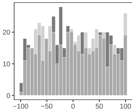
Exponential
