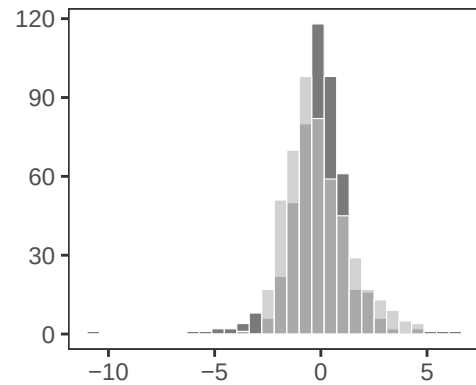
Gamma
