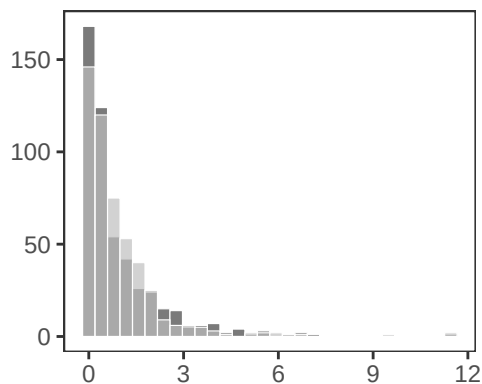
Chi-squared
