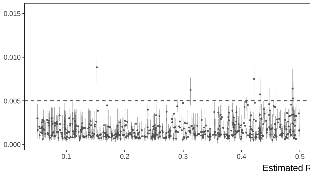
Continuous
