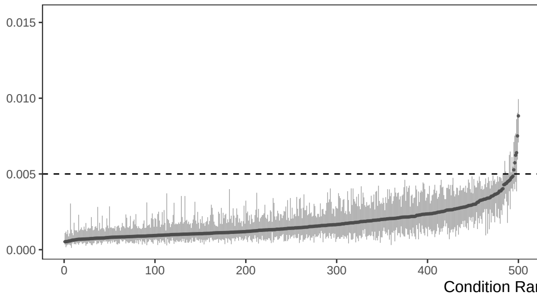
Continuous
