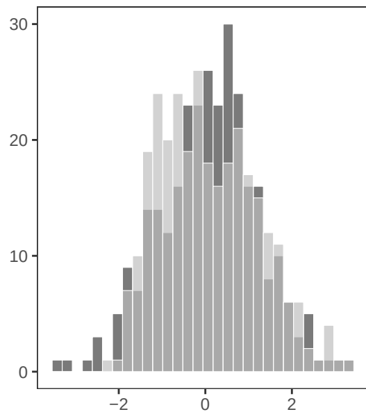
x1 Marginal
