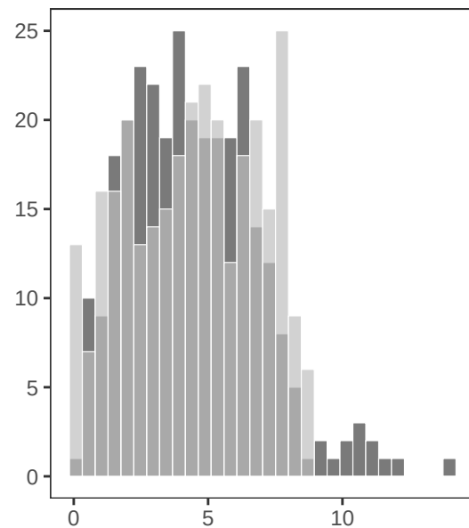
x2 Marginal
