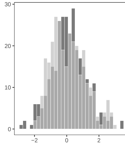
x3 Marginal
