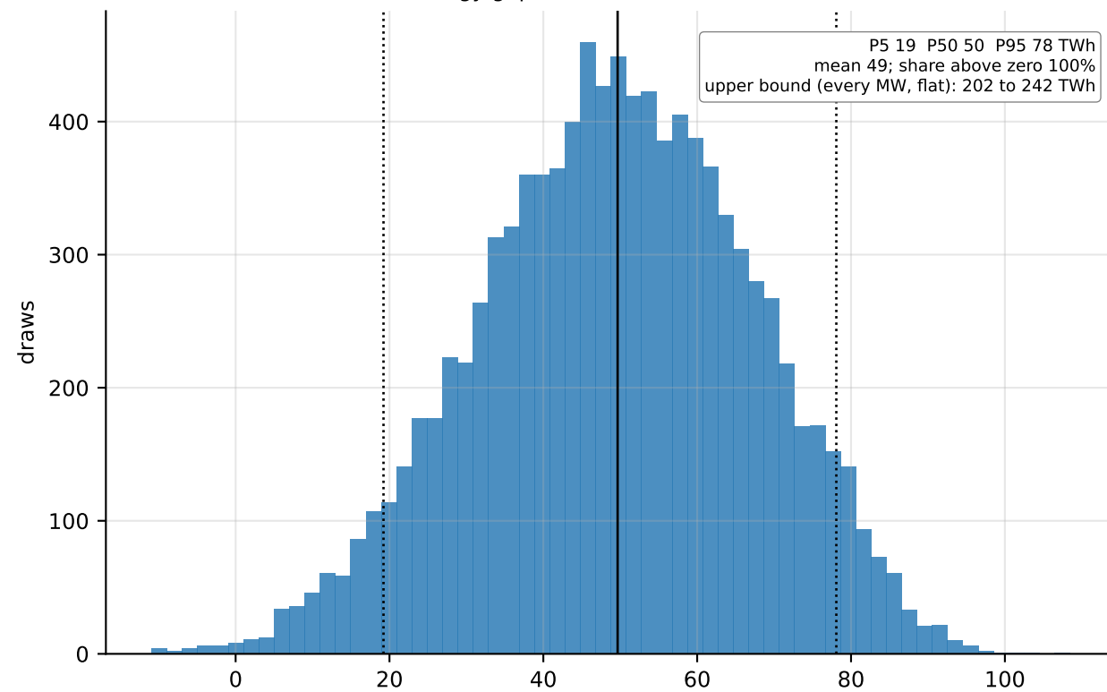
Energy gap in 2030, all 10,000 draws
