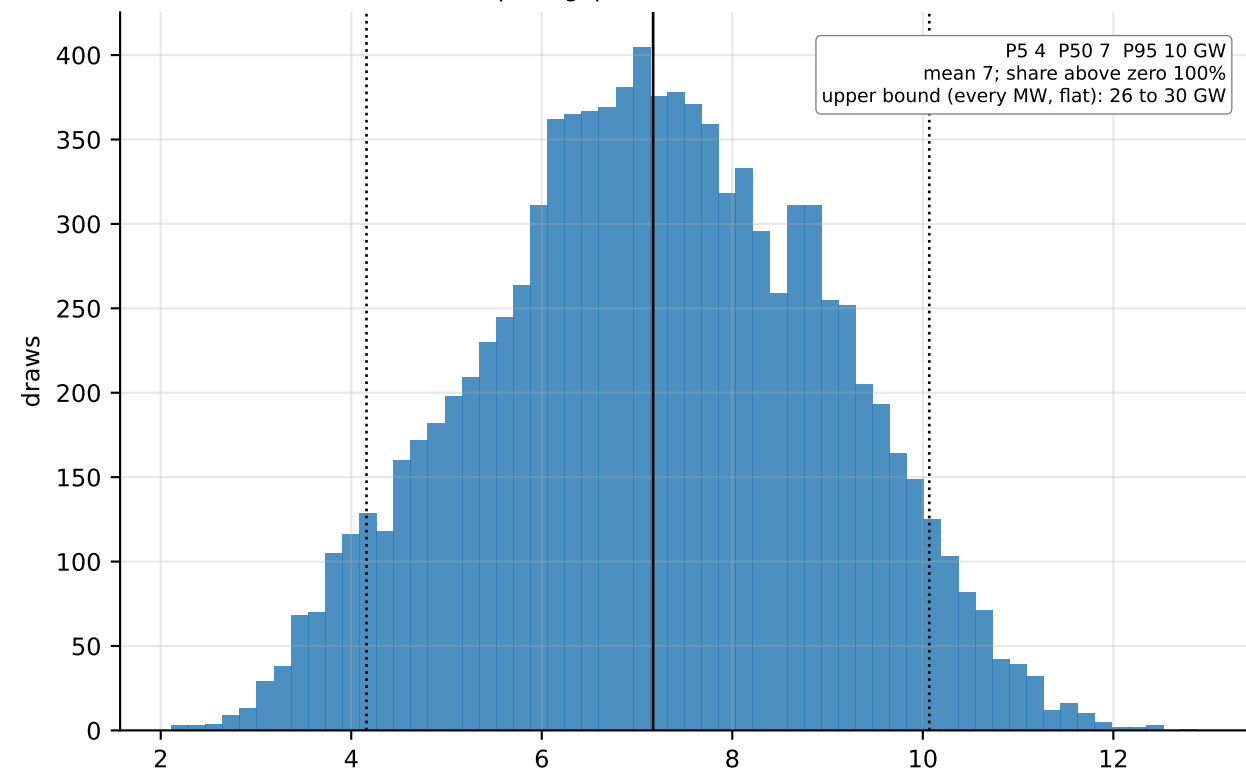
Net-peak gap in 2030, all 10,000 draws
