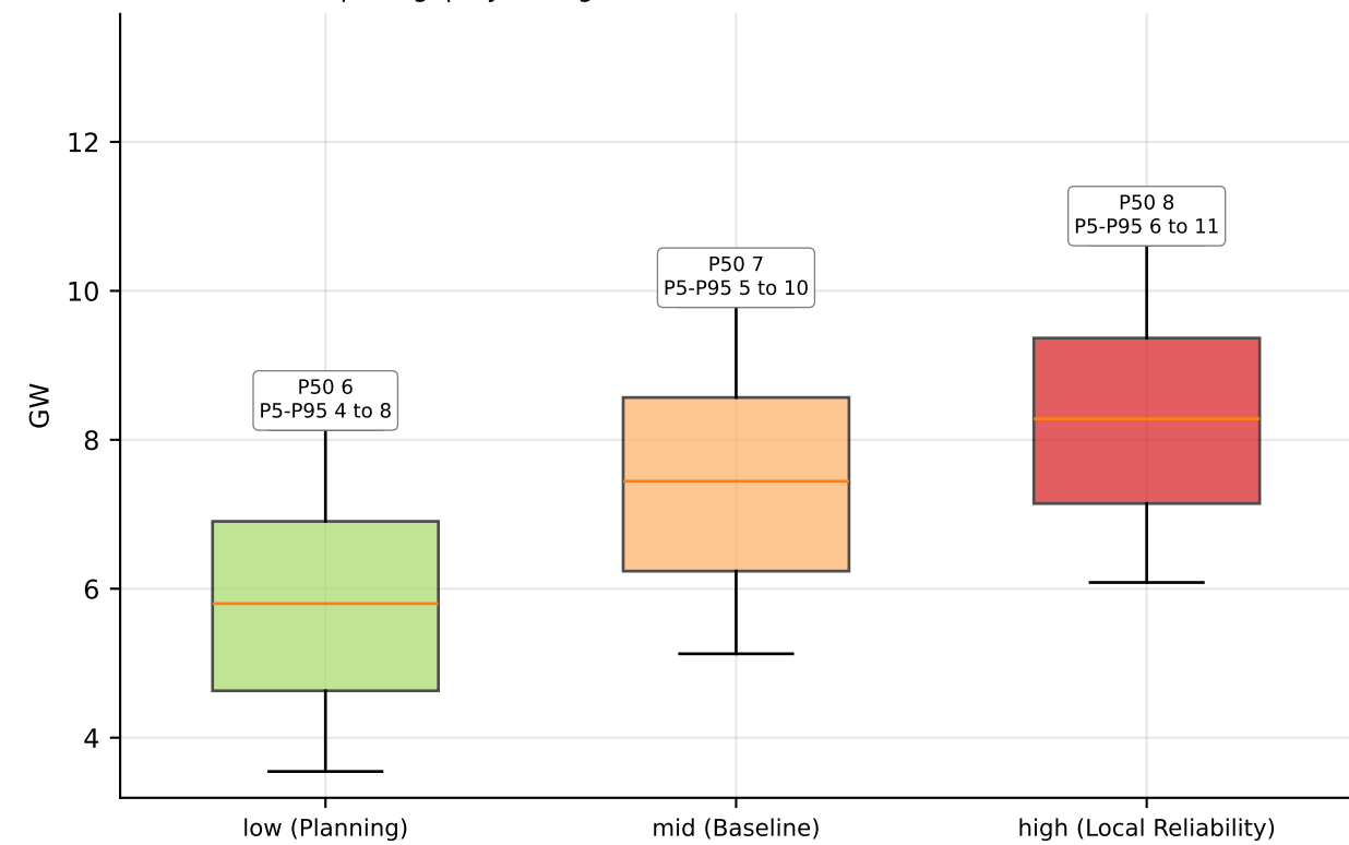
Net-peak gap by IEPR growth case (boxes P25-P75, whiskers P5-P95)
