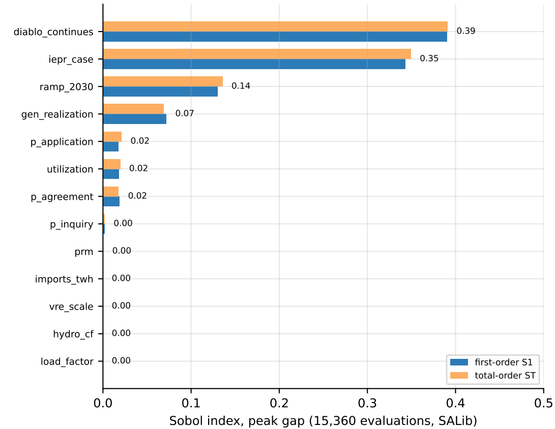
Sobol indices, peak gap (sum of S1 = 0.99)
