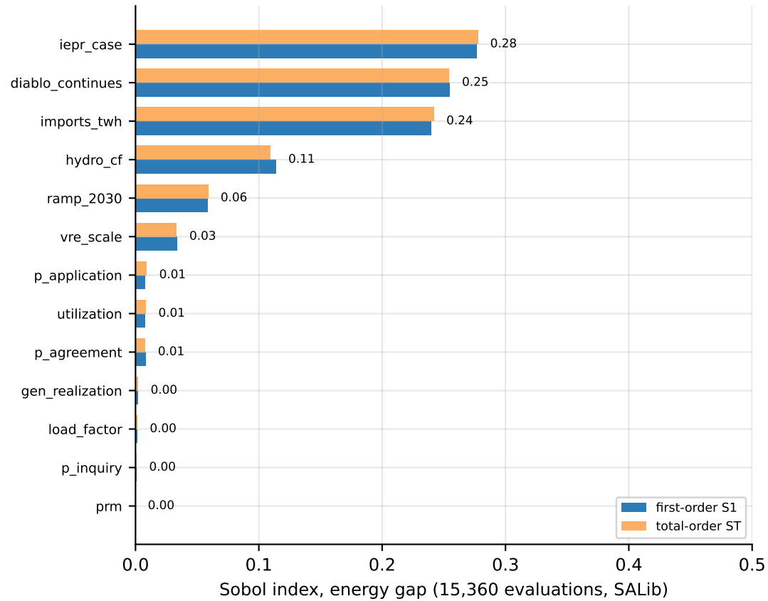
Sobol indices, energy gap (sum of S1 = 1.01)
