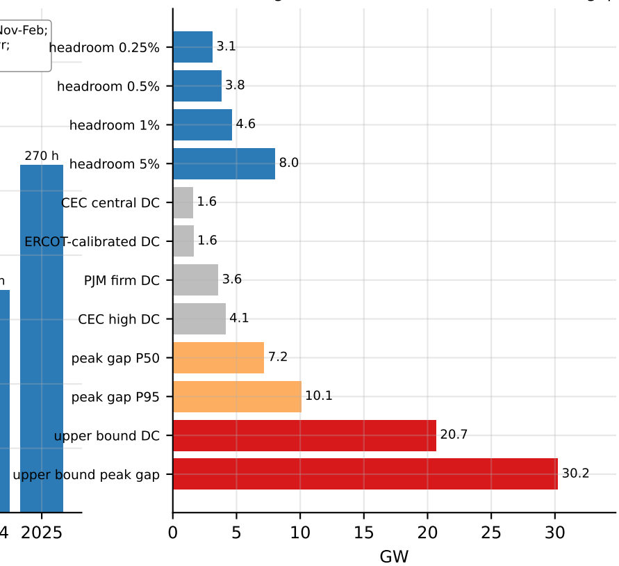
Headroom against the data center cases and the gap
