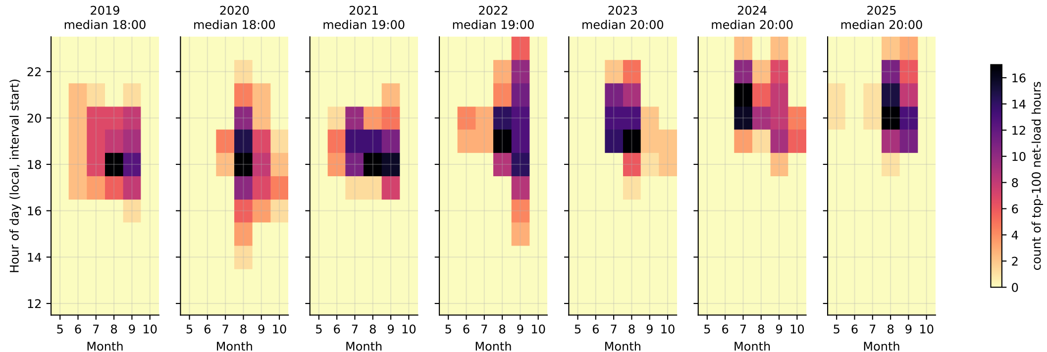
When the 100 highest net-load hours occur, CAISO, by year
