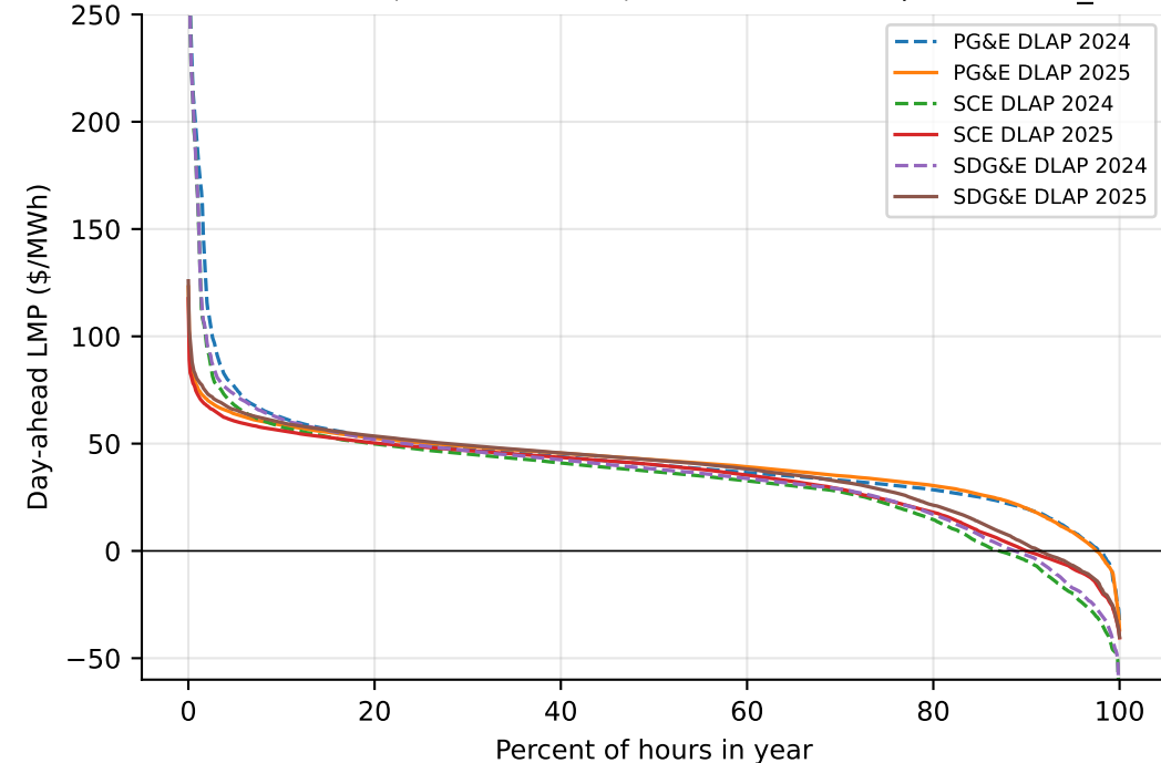
Price duration curves, CAISO DLAPs, 2024 and 2025 (OASIS PRC_LMP DAM)
