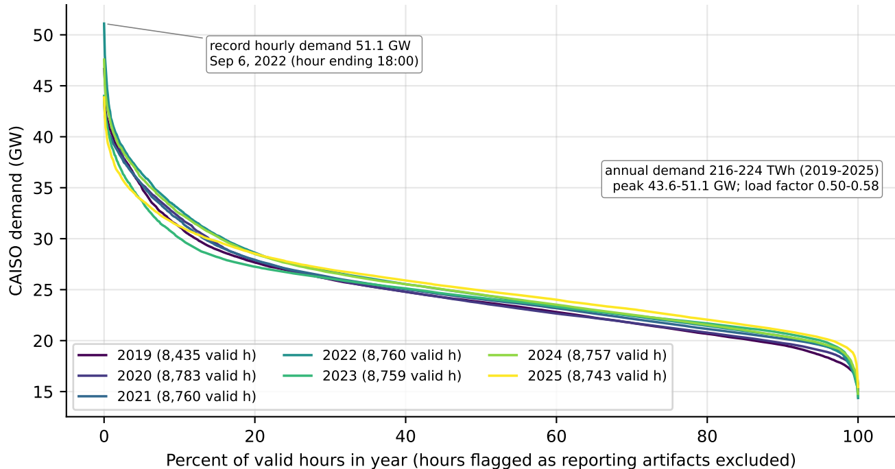
Load duration curves, CAISO balancing authority, 2019-2025 (EIA-930 Adjusted demand)
