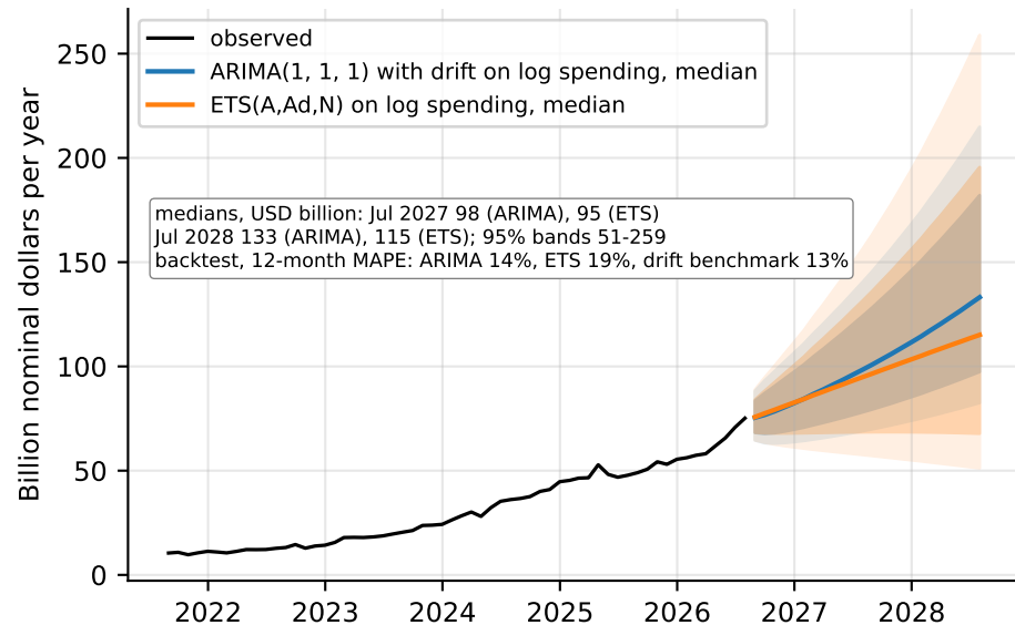
Log-linear trends and breaks (Chow F = 63, p < 0.001 ) 24-month forecasts (back-transformed log medians) with 80% and 95% bands
