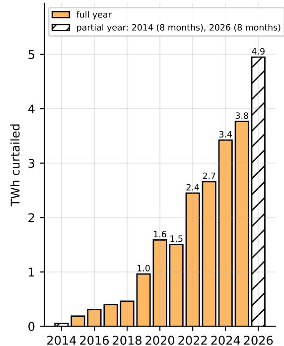
CAISO wind and solar curtailment
