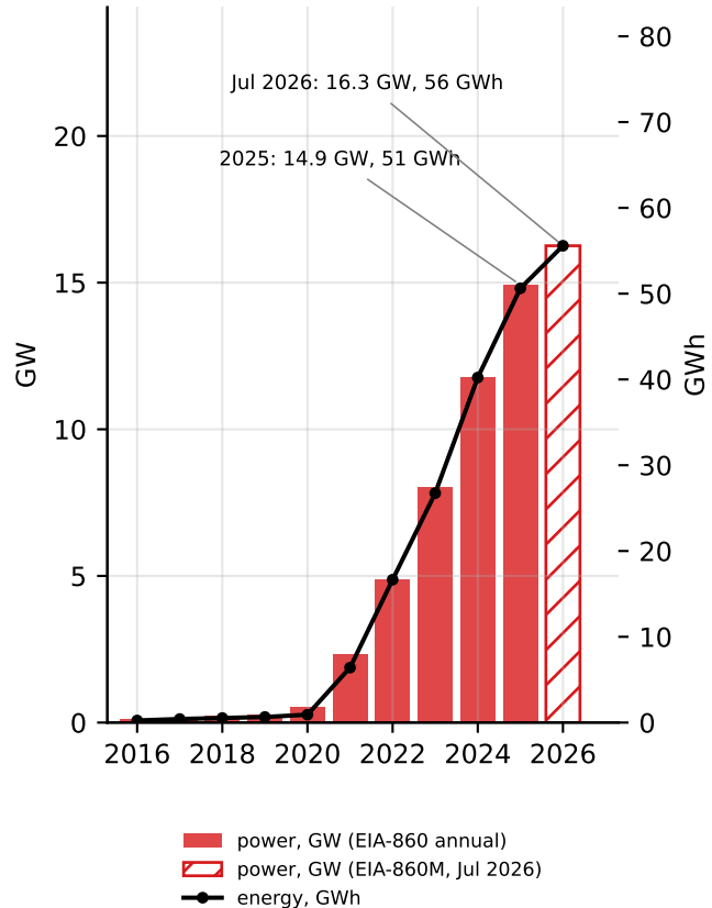
Battery storage, operable (EIA-860)
