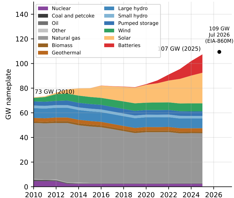
Operable capacity by technology (EIA-860 annual; July 2026 from EIA-860M)
