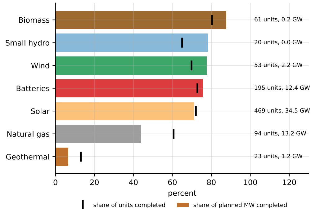
Completion by technology, seven vintages pooled (technologies with 15 or more unit-vintages)
