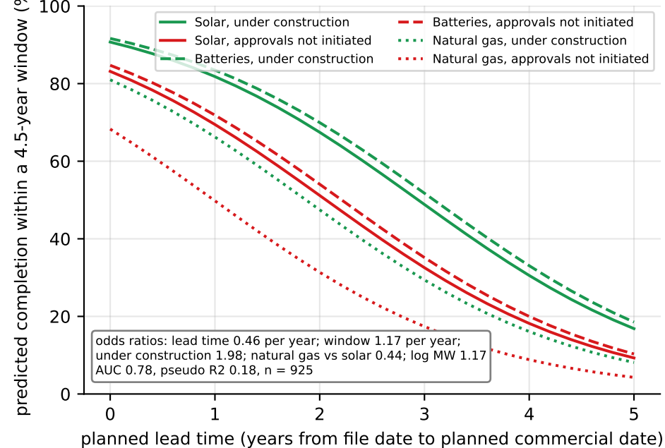
Logistic model, 50 MW unit, window July 2026 to Dec 2030
