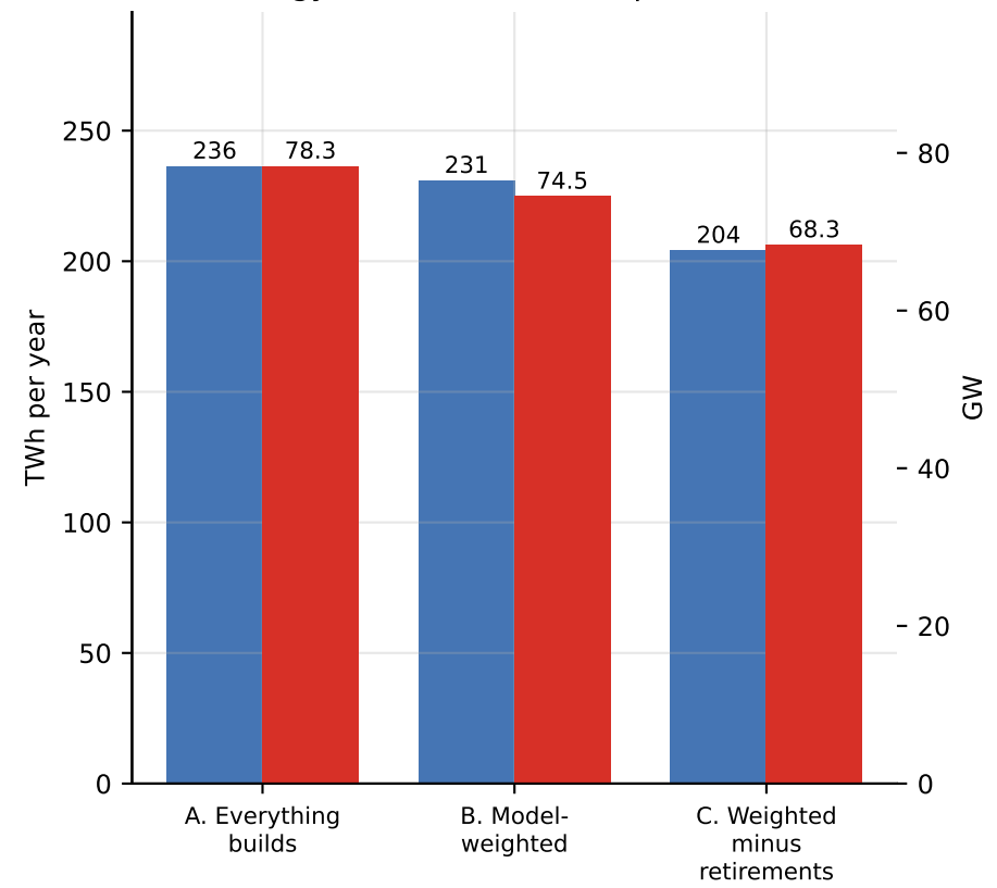
Energy and ELCC-derated peak, 2030
