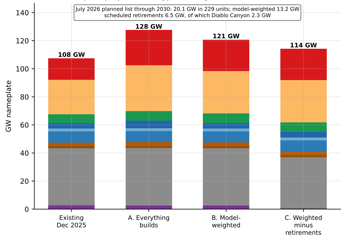
Capacity by technology: existing and three 2030 cases
