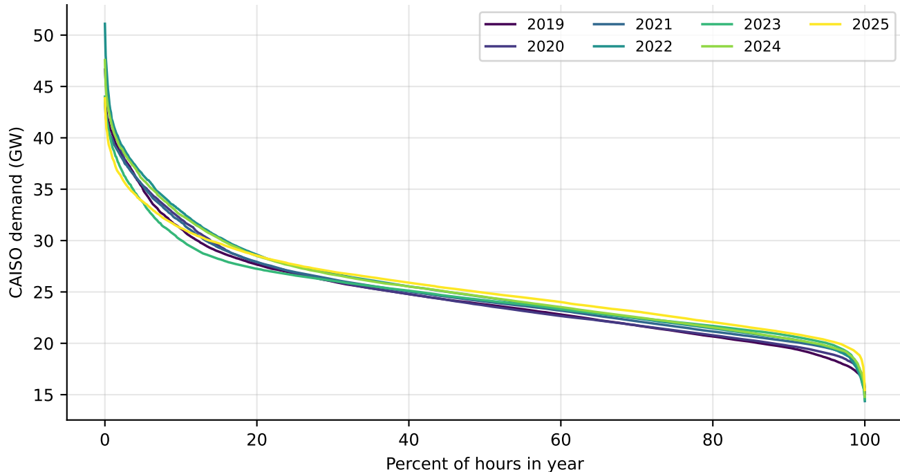
Load duration curves, CAISO balancing authority, 2019-2025 (EIA-930)
