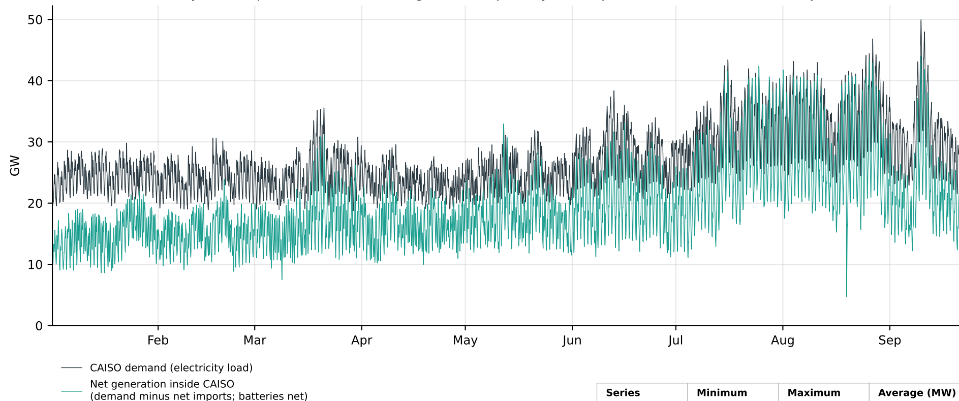
CAISO hourly consumption and in-CAISO net generation, January 1 to September 20, 2026 (EIA-930, adjusted series)
