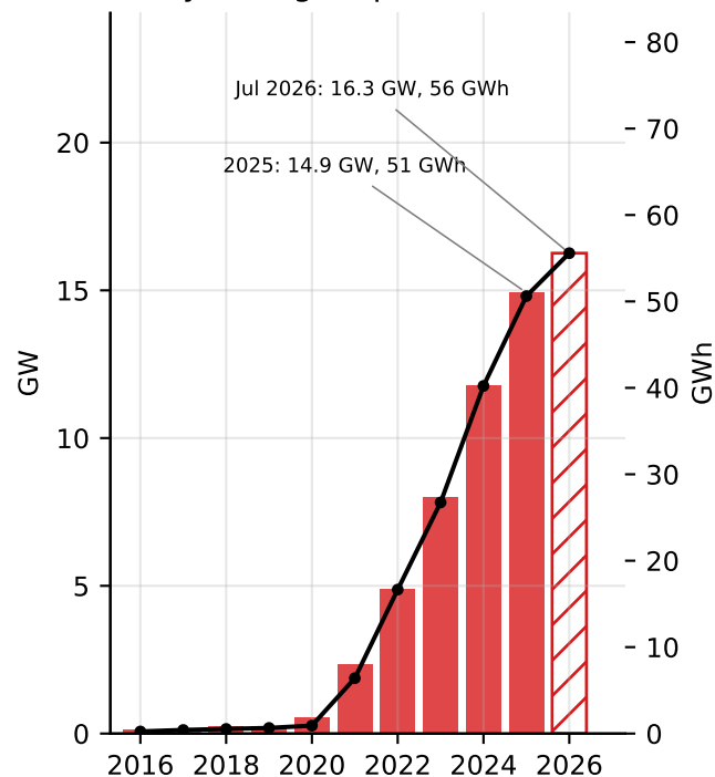
Battery storage, operable (EIA-860)
